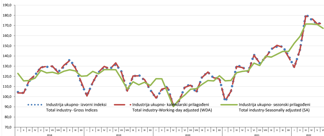
Grafik 1. Vremenska serija industrija ukupno - izvorni, kalendarski i sezonski prilagođeni indeksi: januar 2018. - juni 2022. (2015=100) Graph 1. Time series for total industry - Gross, Working-day and Seasonally Adjusted indices: January 2018 - June 2022 (2015=100)
