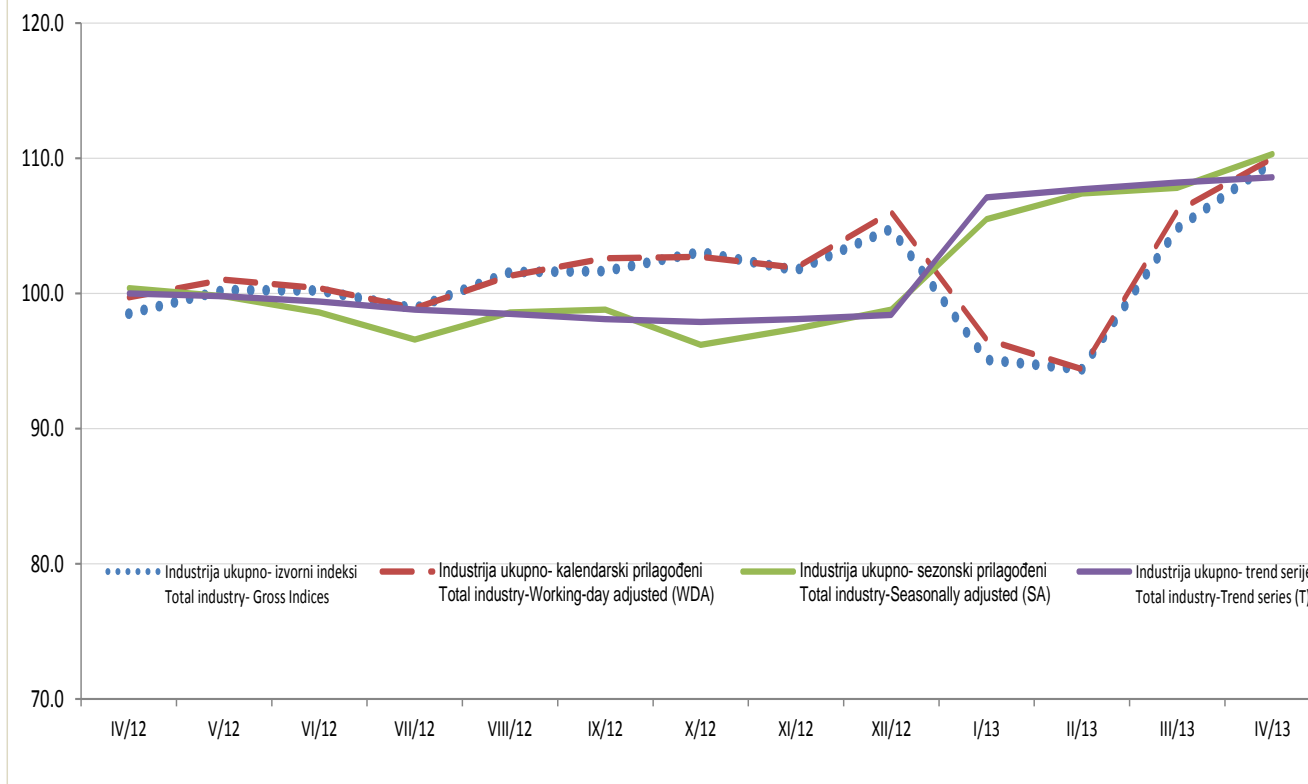
Grafik 1. Mjesečna serija indeksa industrija ukupno - izvorni, kalendarski i sezonski prilagođeni indeksi: april 2012 - april 2013 (2010 = 100) Graph 1. Monthly series of industrial indices for total - Gross, Working-day and Seasonally Adjusted indices: April 2012 - April 2013 (2010=100)
