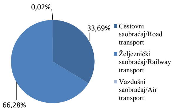
G.2. Struktura prevoza robe, I kvartal 2015. godine Structure of goods transport, first quarter 2015
