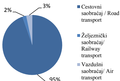
G.1. Struktura prevoza putnika, I kvartal 2015. godine Structure of transport of passengers, first quarter 2015
