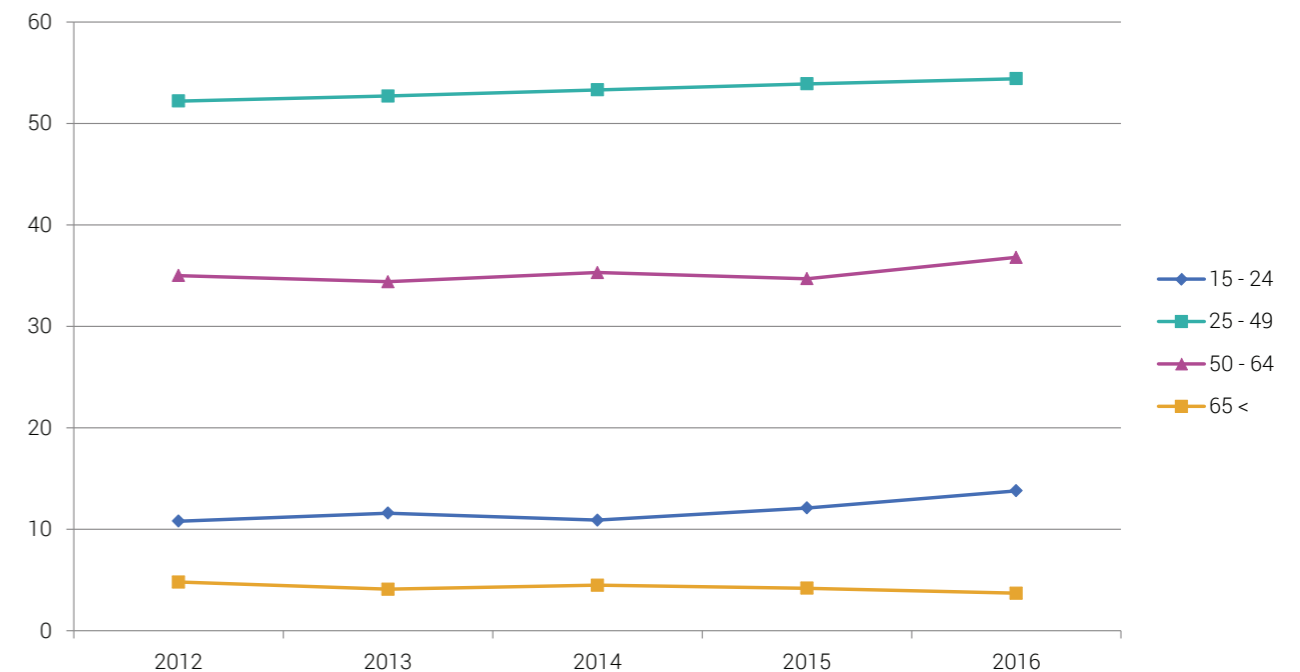
Grafikon 3. Stopa zaposlenosti po starosnim grupama, 2012-2016. Graph 3. Total employment rate by age groups, 2012-2016
