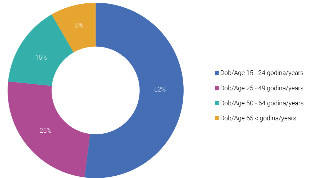
Grafikon 6. Stopa nezaposlenosti po starosnim grupama, 2016, % Graph 6. Total unemployment rate by age group, 2016, %
