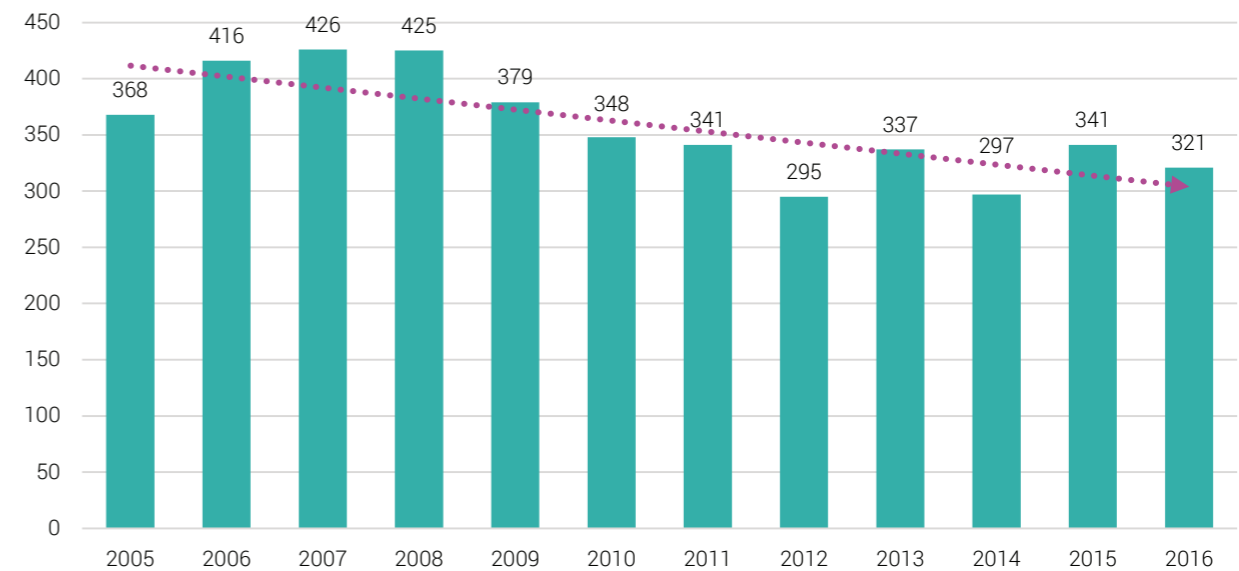
Grafikon 21. Broj poginulih u saobraćajnim nezgodama Graph 21. People died in road accidents
